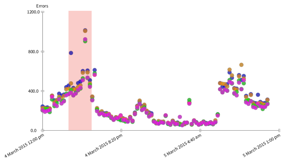
All errors from the log files. Each circle denotes 15 minutes worth of errors. The color of the circle denotes a distinct server node.
