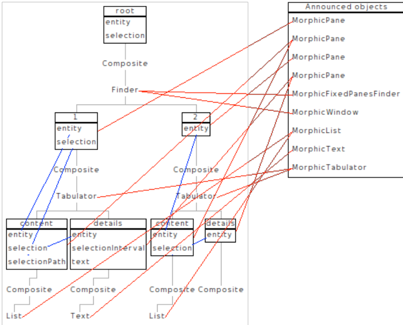
the initial visualization how the objects to the right are connected to more objects from the left
